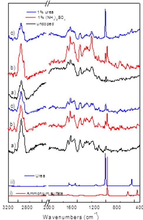
Fig 9. FT-Raman spectra of bloodmeal fertilizers i) ammonium sulphate; ii) urea and bloodmeal fertilizer a) undoped; b) doped with 1% ammonium sulfate and c) doped with 1% urea.
