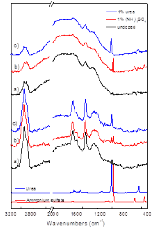
Fig 10. FT-Raman spectra of feathermeal fertilizers a) undoped; b) doped with 1% ammonium sulfate and c) doped with 1% urea.
