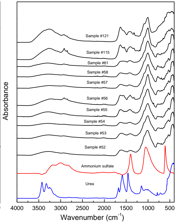
Fig 5. ATR_FTIR spectra of organic compost fertilizers.
