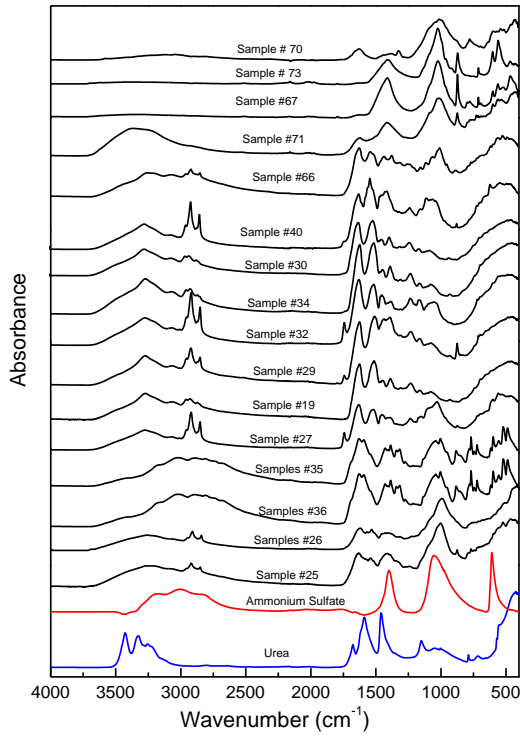
Fig 4. ATR_FTIR spectra of selected guano fertilizers
