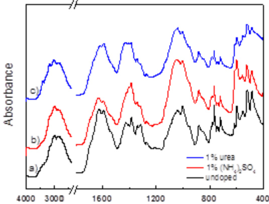
Fig 10. ATR-FTIR spectra of seabird guano a) undoped; b) doped with 1% ammonium sulfate and c) doped with 1% urea.
