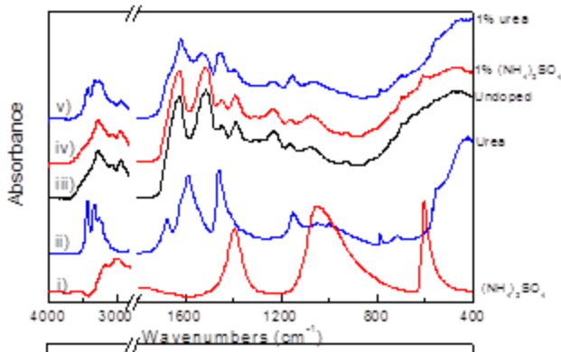
Fig 8. ATR-FTIR spectra of i) ammonium sulphate; ii) urea and bloodmeal fertilizer iii) undoped; iv) doped with 1% ammonium sulfate and v) doped with 1% urea.
